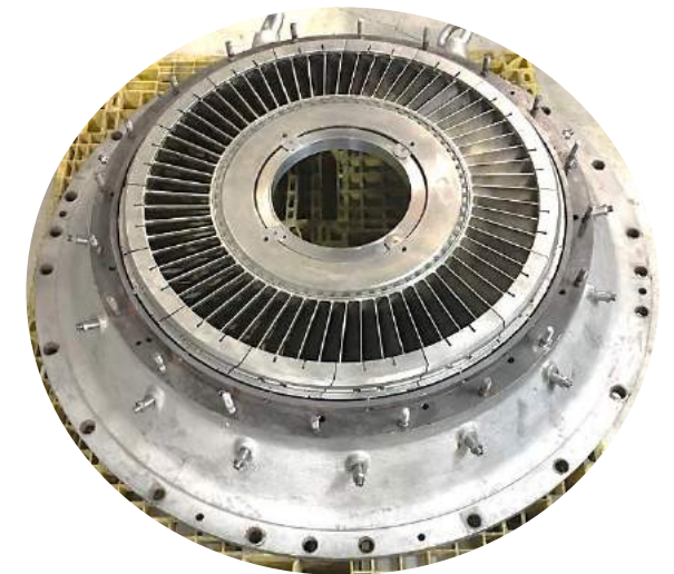
Power Turbine (PT) Stator Assembly
