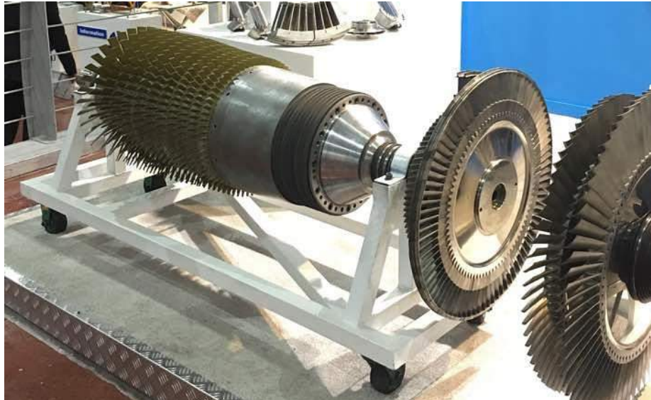
Gas Generator (GG) Turbine Rotor
